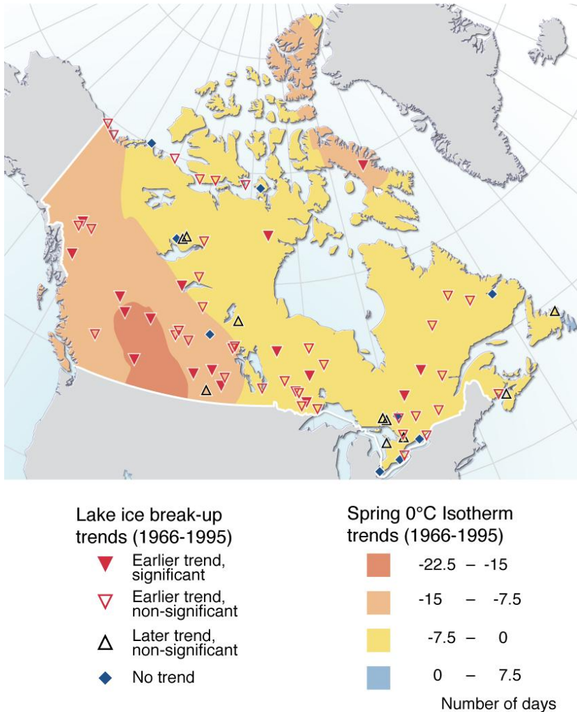
Figure 7.1. Trends in lake ice break-up and spring 0°C isotherms over Canada from 1966-1995. Similar spatial and temporal patterns are found between the two trends, with the most significant trends towards earlier springs and earlier break-up dates over most of western Canada. (Source: UNEP/GRID-Arendal. Trends in spring temperatures and ice break-up dates in Canada. UNEP/GRID-Arendal Maps and Graphics Library.)
