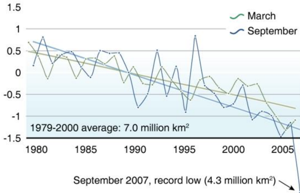
Figure 5.1. Anomalies in sea-ice extent compared to the 1979-2000 average of 7.0 million km 2 in September and 15 million km 2 in March. (Source: UNEP/GRID-Arendal, 2007. Trends in Arctic sea ice extent in March (maximum) and September (minimum) in the time period of 1979–2007. UNEP/GRID-Arendal Maps and Graphics Library.)
