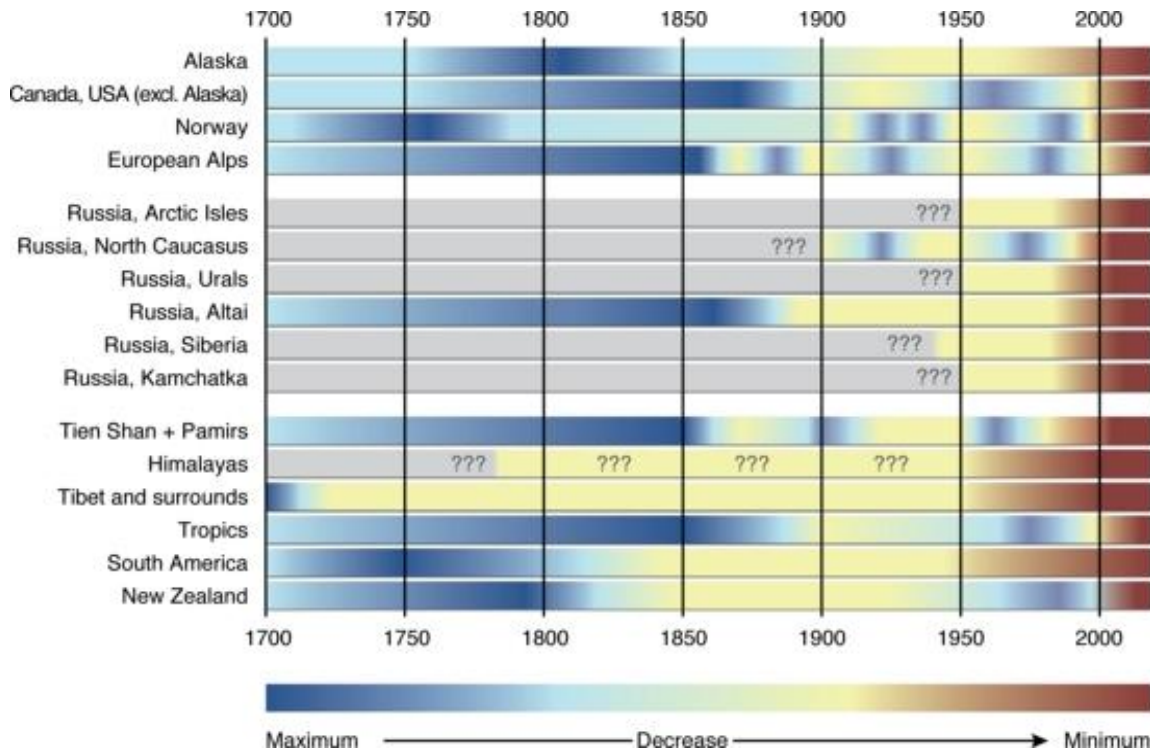
Figure 4.1. Overview of regional glacier changes since the end of the Little Ice Age (early 14 th to mid 19 th century). (Source: UNEP/GRID-Arendal. 2007. Overview on glacier changes since the end of the Little Ice Age. UNEP/GRID-Arendal Maps and Graphics Library.)
