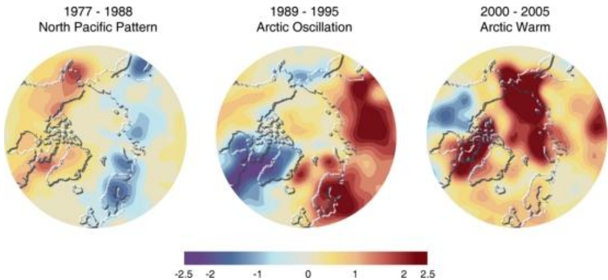
Figure 2.3. Recent Northern Hemisphere surface temperature anomalies averaged over periods with different dominant patterns of natural variability. The pattern of warm temperature anomalies in recent years (2000-2005) does not match either of the two previous climate patterns. (Source: UNEP/GRID-Arendal. 2007. Arctic temperature anomaly patterns. UNEP/GRID-Arendal Maps and Graphics Library.)
