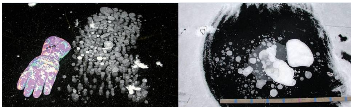
Figure 9.2. Methane bubbles trapped in lake ice form distinct patterns as a result of differing rates of methane bubbling. In Walter et al. (2006), methane emissions from the entire lake were estimated by surveying the distribution of bubble patterns in lake ice in early winter. (Source: UNEP/GRID-Arendal. 2007. Global Outlook for Ice and Snow)
