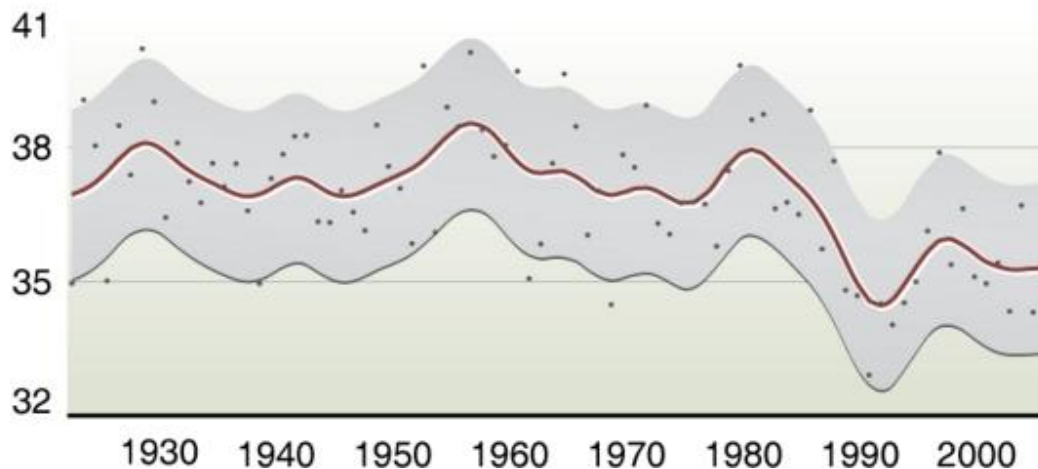
Figure 6.1. Northern Hemisphere snow-covered area (SCA) for the spring (March-April) from 1922-2005. Since the early 1920s, and especially since the late 1970s, SCA has declined in the spring. The linear trend shows a decrease in snow-covered area of 2.7 \pm 1.5 \times 10^6 km 2 or 7.5 \pm 3.5\% . The shaded fields in the figure represent the 5 to 95% range of the data. (Source: UNEP/GRID-Arendal. Trends in snow-covered area for the Northern Hemisphere 1922-2005. UNEP/GRID-Arendal Maps and Graphics Library.)
