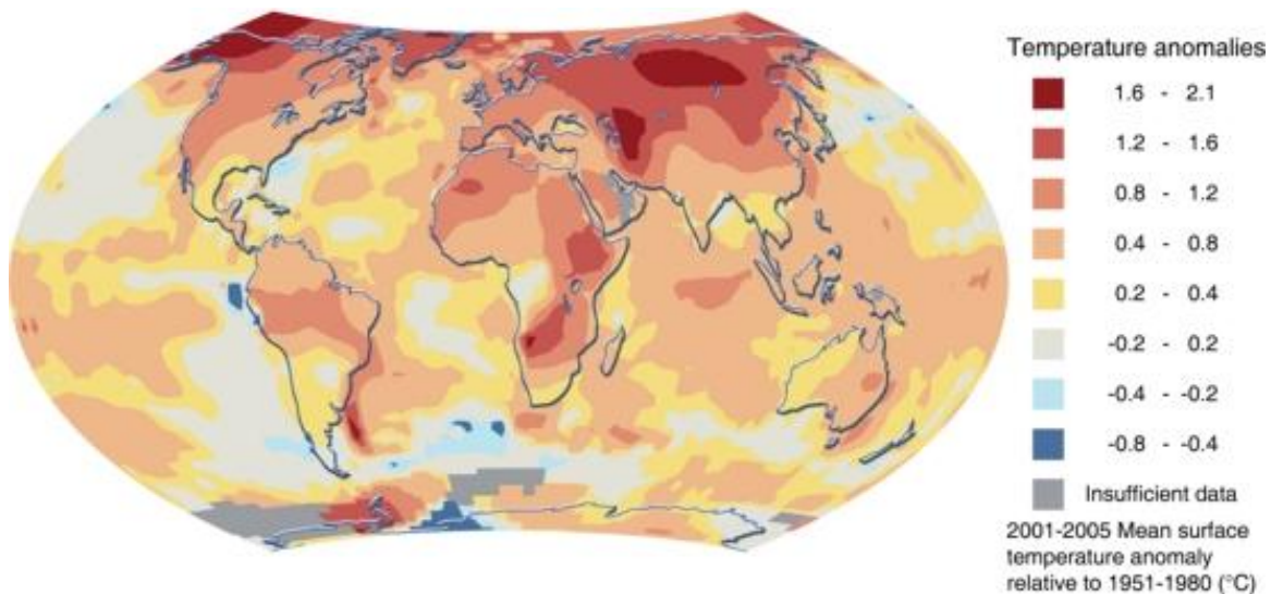
Figure 2.2. Increases in annual temperatures for 2001-2005 relative to 1951-1980, showing the greatest warming over land and at high latitudes in the Northern Hemisphere. (Source: UNEP/GRID-Arendal. 2007. Increases in annual temperatures for a recent five-year period, relative to 1951-1980. UNEP/GRID-Arendal Maps and Graphics Library.)
