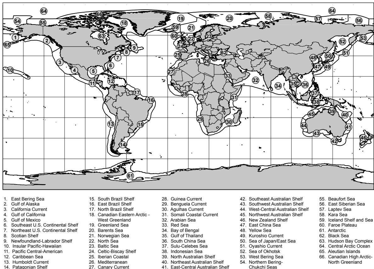
Fig. 15 Large marine ecosystems considered in this study.
